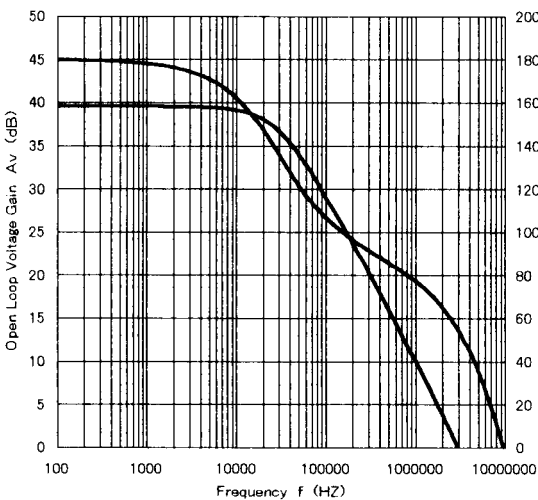
NJM13403 Open Loop Voltage Gain vs. Frequency
